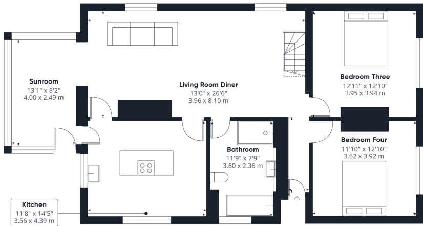
Floor 0
